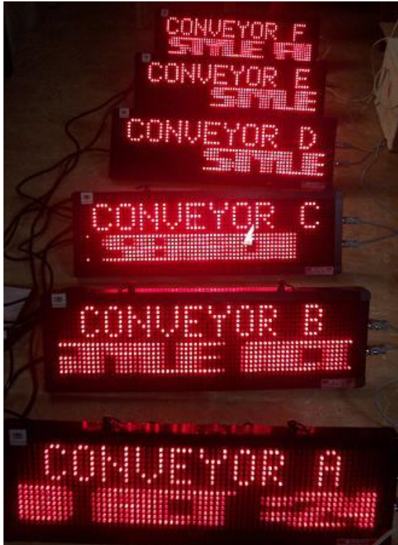
Multiple boards on a RS485 loop, controlled from a Single PC or individually from a PC Keyboard
